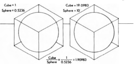
The relationship of cube to inscribed sphere.
